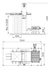
Pallet Version: 120/100/80x120
