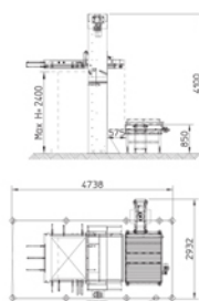
Pallet Version: 100/80x120
