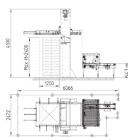
Pallet Version: 120/100/80x120
