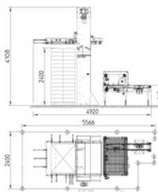
Pallet Version: 100/80x120
